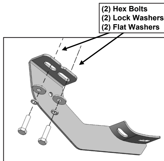
(Figure 8) Attach Passenger/Right Center/Rear Mounting Brackets.
