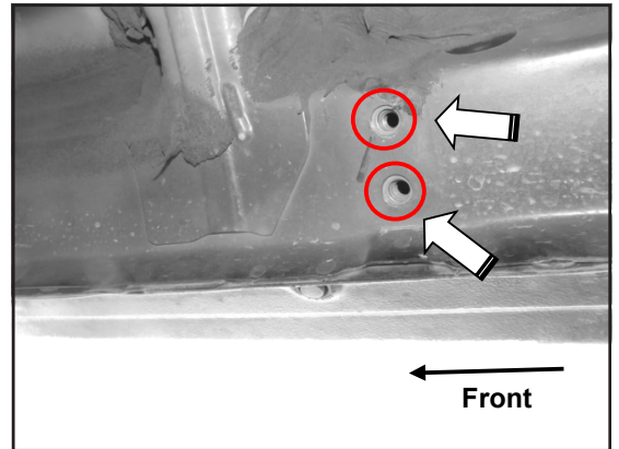
(Figure 4) Attach Passenger/Right Center/Rear Mounting Bracket to Center threaded inserts until hand tight.
