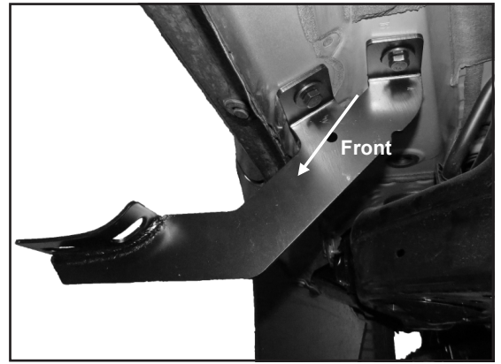
(Figure 3) Attached Passenger/Right Front Mounting Bracket at Front Mounting Location.
