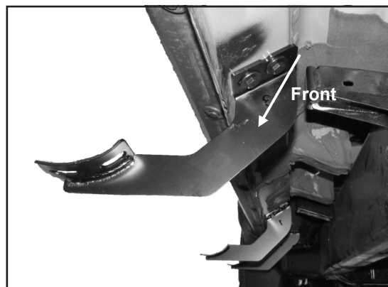
(Figure 9) Attached Passenger/Right Center/Rear Mounting Bracket at Rear Mounting Location.
