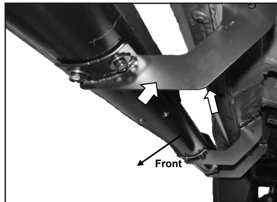
(Figure 11) Attached Side Bar on all Passenger/Right Brackets.
