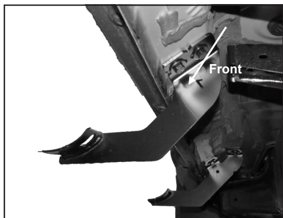
(Figure 6) Attached Passenger/Right Center/Rear Mounting Bracket at Center Mounting Location.
