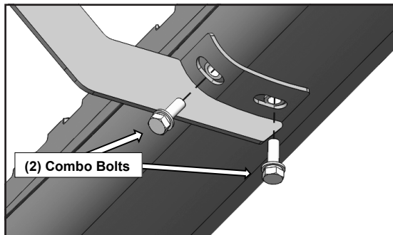
(Figure 10) Attach Side Bar to all Passenger/Right Brackets until hand tight.
