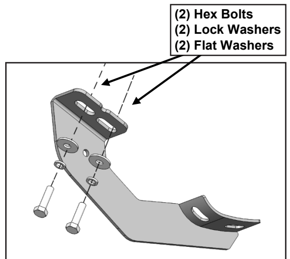
(Figure 5) Attach Passenger/Right Center/Rear Mounting Bracket.
