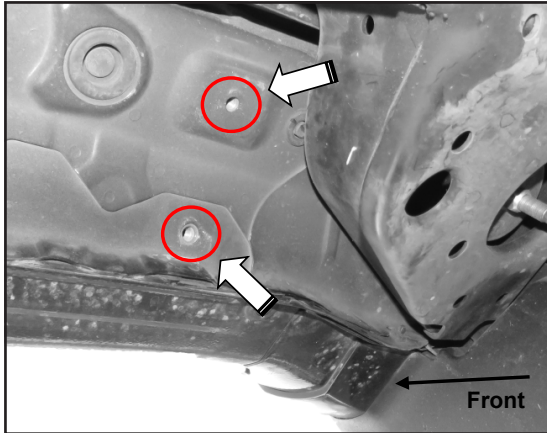
(Figure 1) Attach Passenger/Right Front Mounting Bracket to Front threaded inserts until hand tight.
